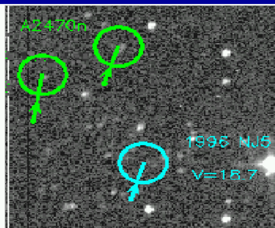
Pass 3: Known object identified, but displaced from expected position
